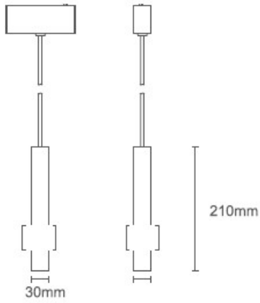
Sizes drawing
