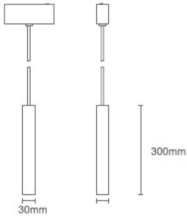
Sizes drawing
