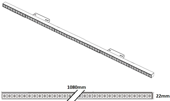
Sizes drawing
