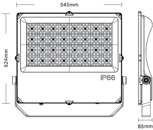
Sizes drawing
