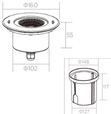
Sizes drawing
