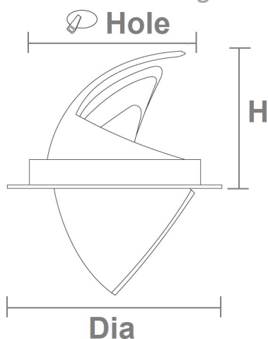
Sizes drawing
