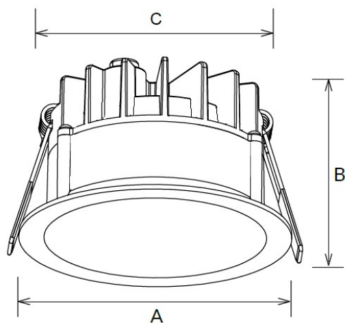
Sizes drawing
