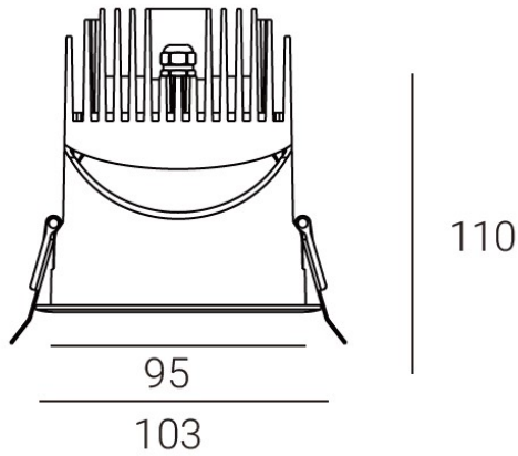
Sizes drawing
