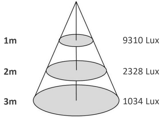
DWR95-MD-SF-C-20W.lux
