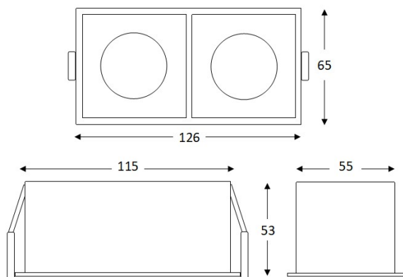
Sizes drawing
