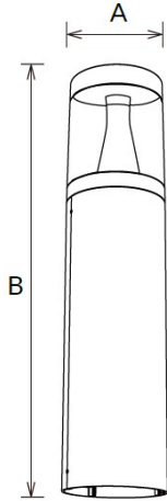
Sizes drawing
